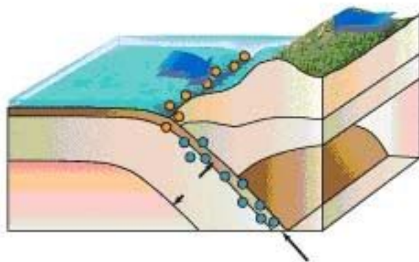
SUBDUCTION ZONE BOUNDARY
