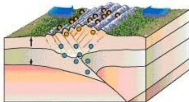
CONTINENTAL COLLISION BOUNDARY
